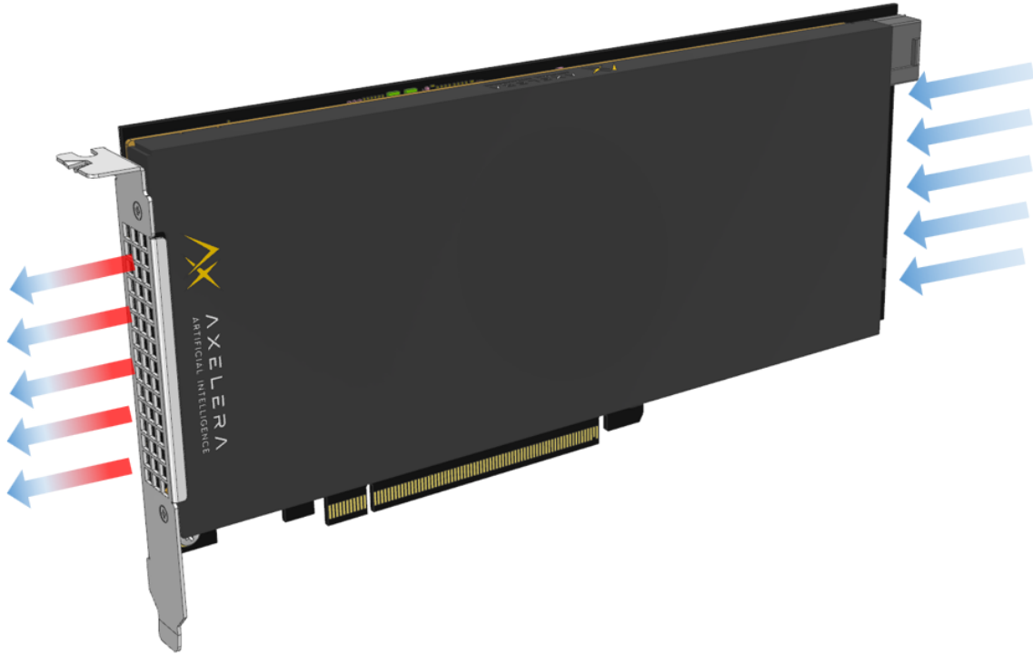
Figure 6: Air flow directions for the Axelera Server 150p with the passive cooling solution
