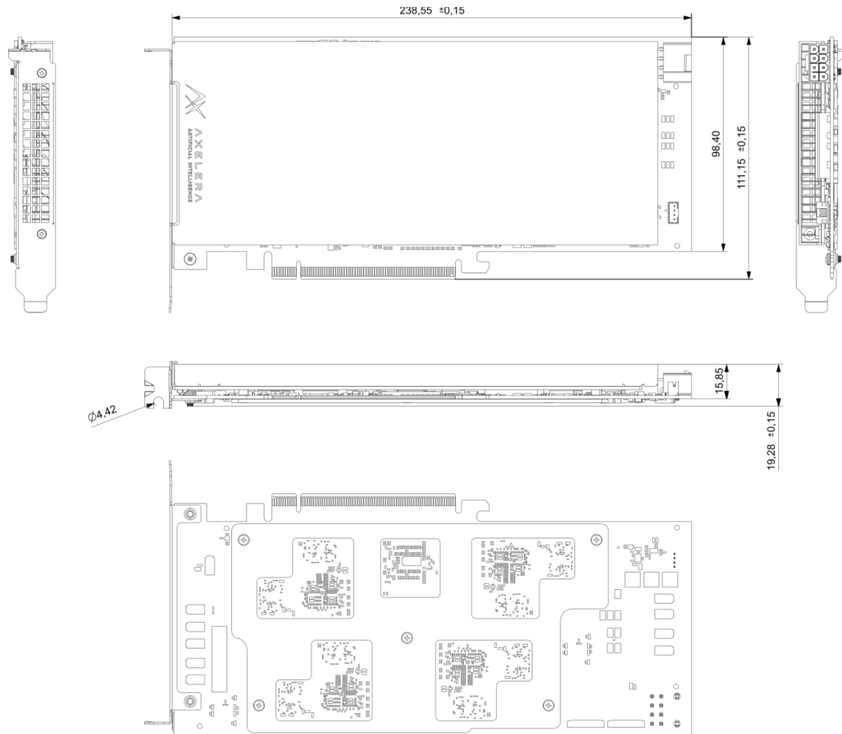
Figure 4: Axelera Server 150p package diagram showing passive cooler
