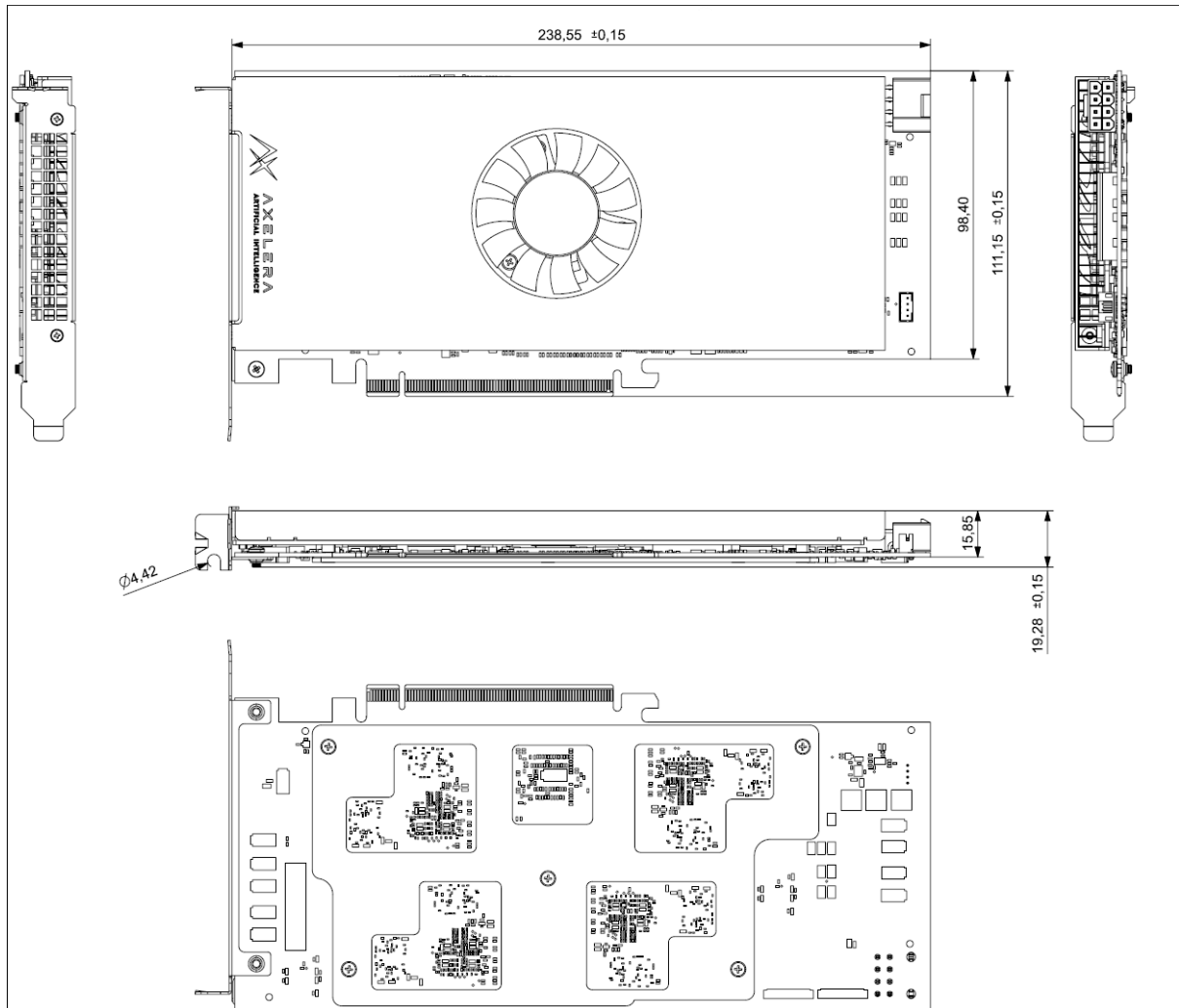
Figure 3: Axelera Server 150p package diagram showing fan-based cooler
