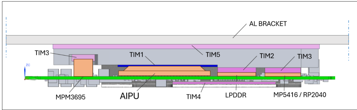
Figure 9: Stack-up of the Axelera Embedded 110m Passive Cooling solution showing the heat spreader in an embedded fan-less system
