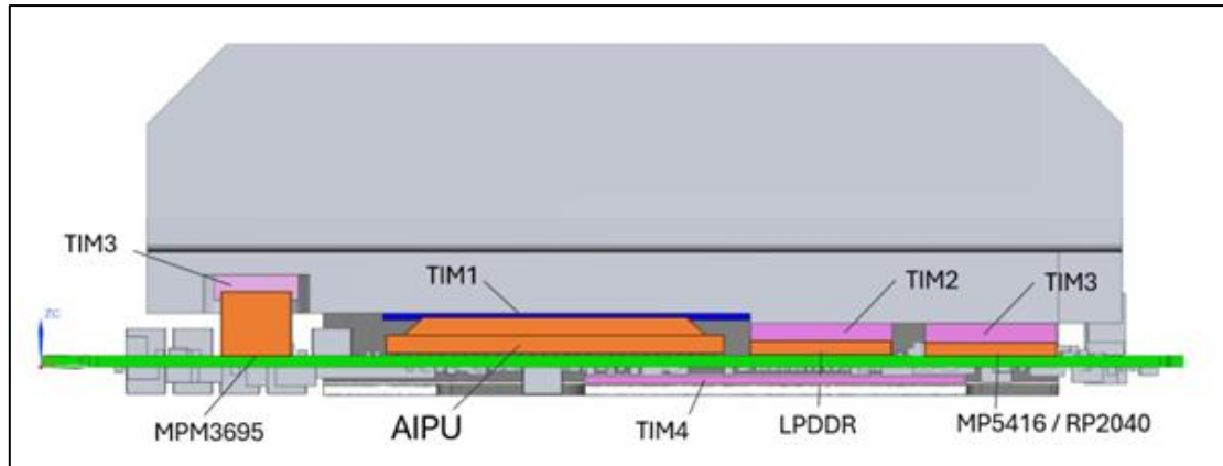
Figure 2: Stack-up of Axelera Embedded 110m (cross-section of AI Heatsink Solution with TIM materials)
